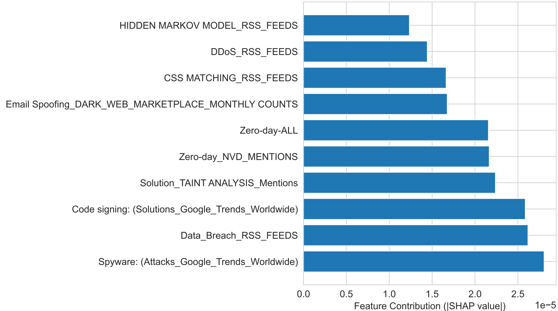
Local Explanation for Sample 0
